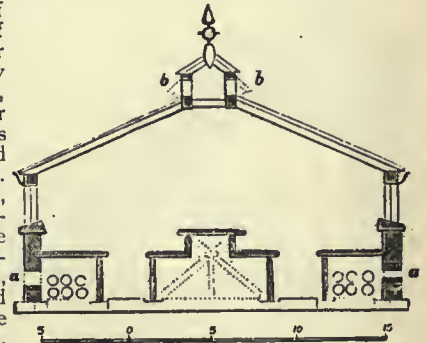
FIG. 4.—Section of Plant Stove.
